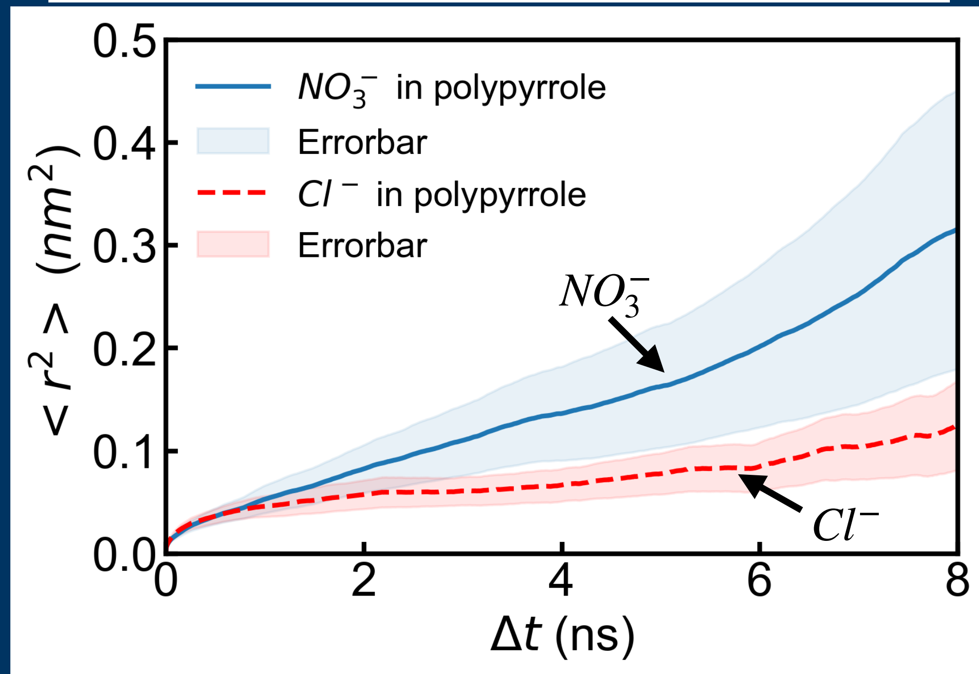
Mean square displacement of NO_3^- and Cl^- in polypyrrole
